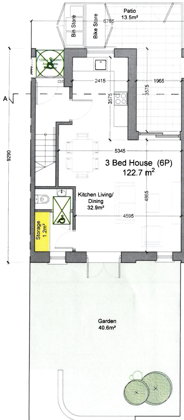
GROUND FLOOR - GIA 43.3m 2
