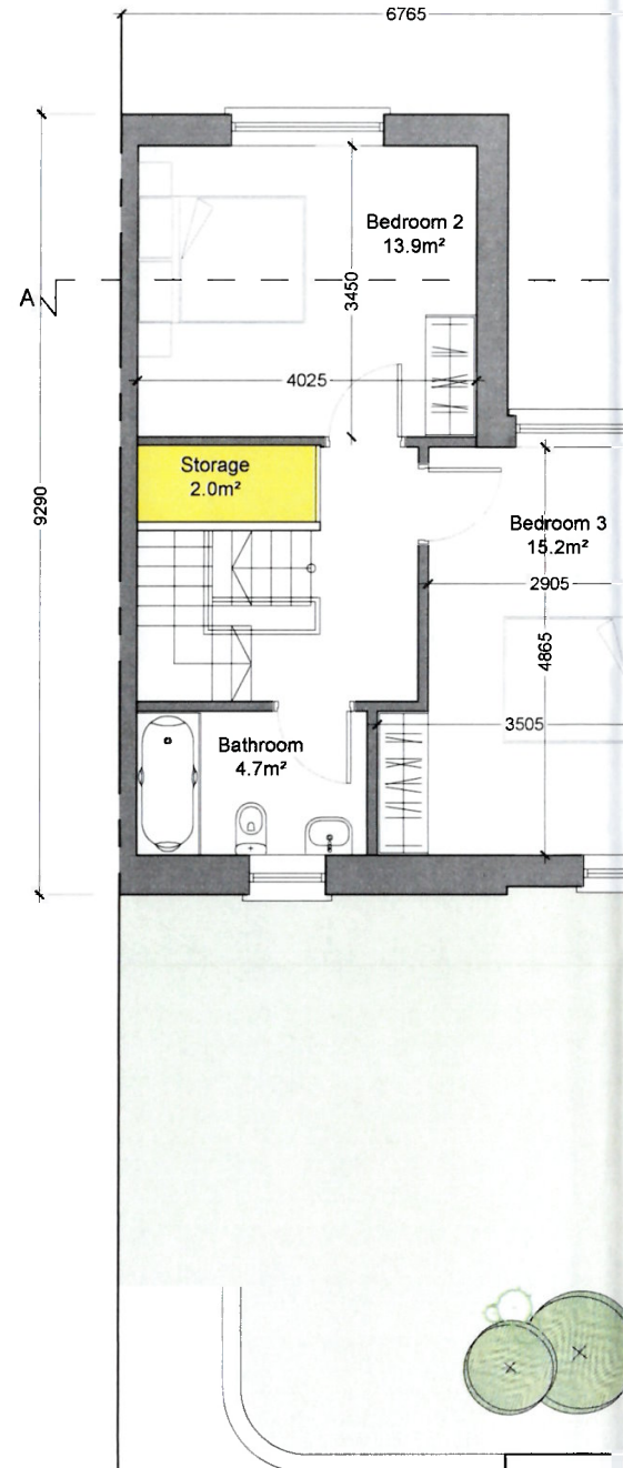
FIRST FLOOR - GIA 45.4m 2
